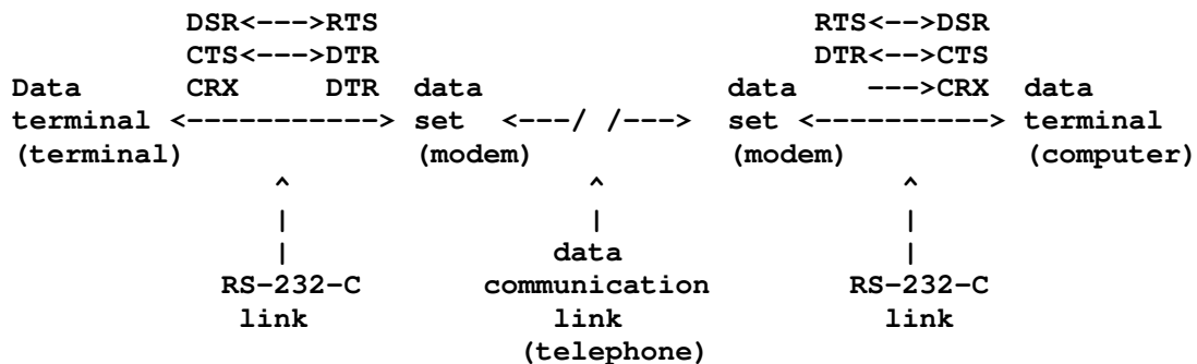
FIGURE 1: COMMUNICATIONS HOOK-UP SHOWING ROLE OF RS-232-C
